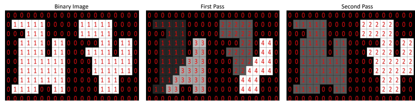
Fig. 3. Demonstration of 2 Pass Connected Component algorithm.
